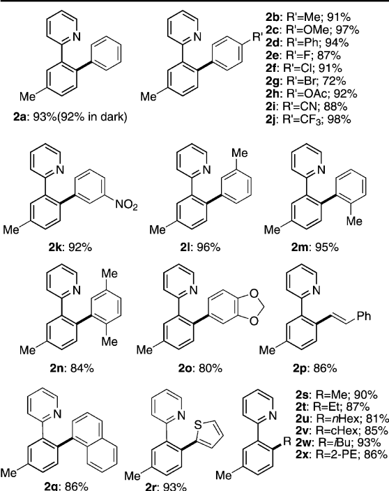
Scheme 2. Extrusion of CO by pyridine-directed rhodium(I)-catalyzed carbon–carbon bond activation. The reactions were carried out using 0.2 mmol of 1 in the presence of 5.0 mol % catalyst in 2.0 mL of PhCl at 140 °C. For experimental details see the Supporting Information. Reported yield is that of the isolated product. 2-PE = 2-phenylethyl.
